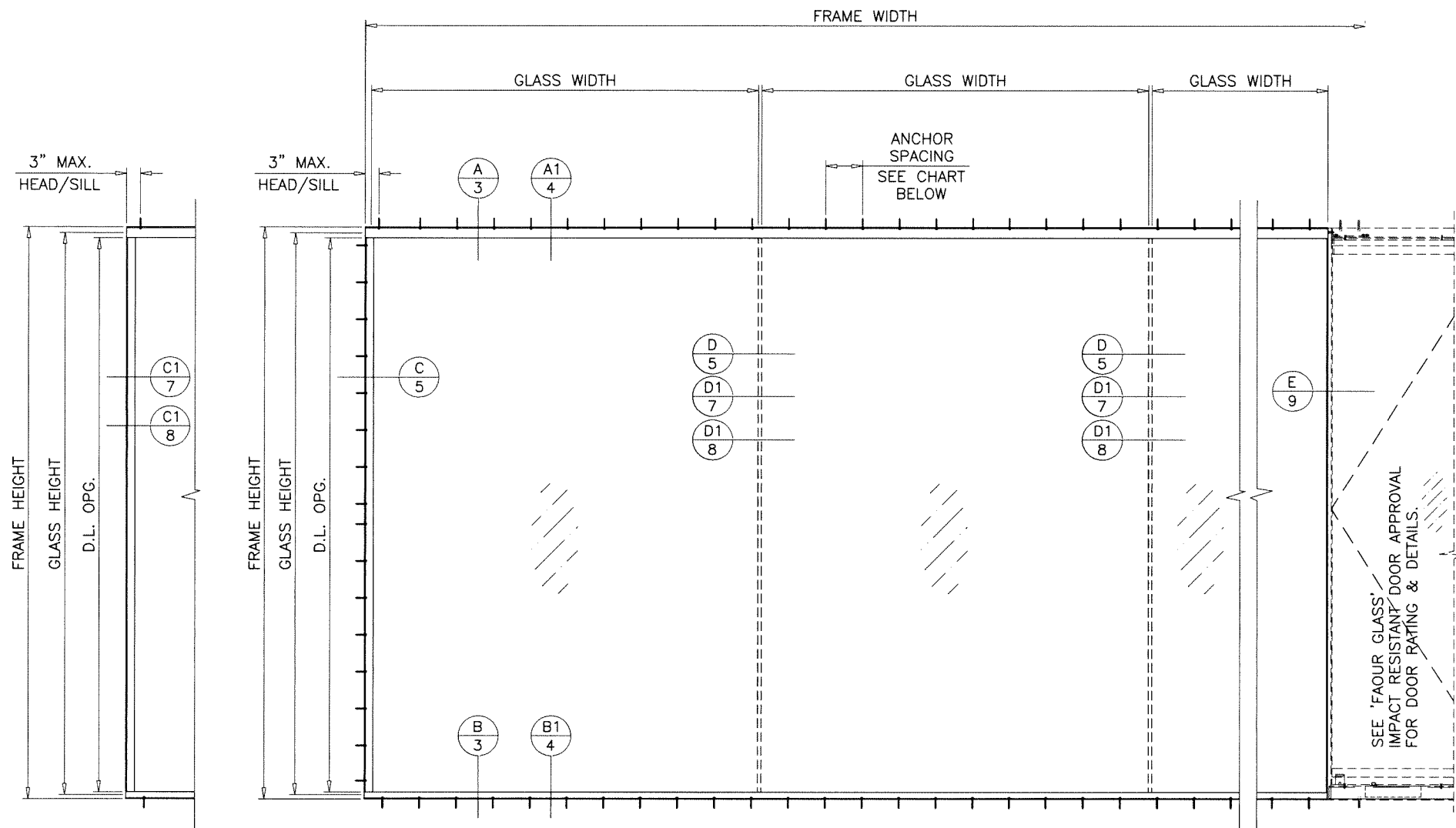
TYPICAL ELEVATION
